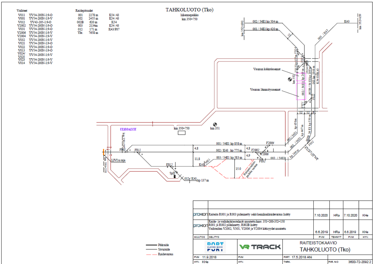
Railway diagram: Tahkoluoto
